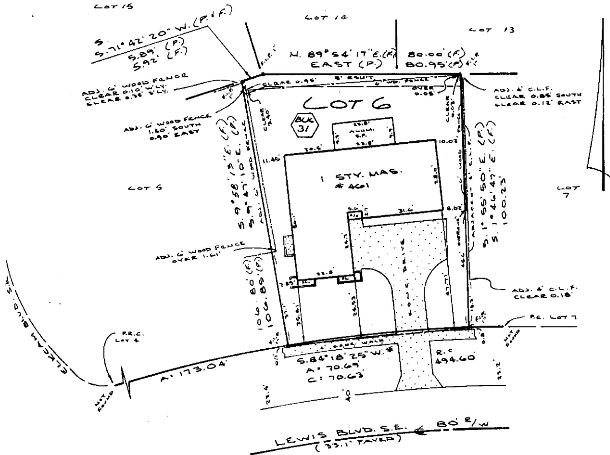
A BOUNDARY SURVEY OF: Lot 6, Block 31, LEWIS ISLAND BAHAMA ISLES ADD, as recorded in Plat Book 58, Pages 95 and 96 of the Public Records of Pinellas County, Florida.
